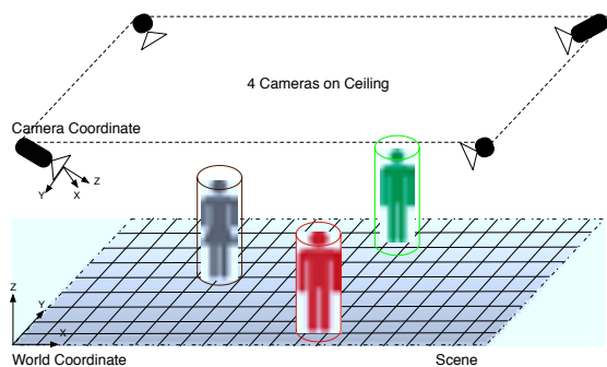
Figure 1: Hardware setup.
